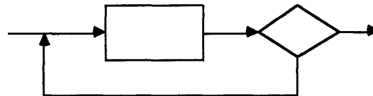
Fig 17 UNTIL Construct
